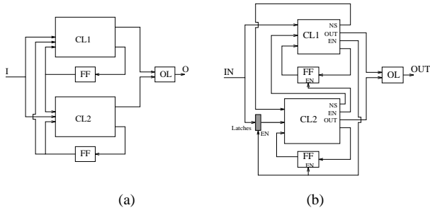
Fig. 4. FSM general decomposition: (a) traditional, (b) with power management.
