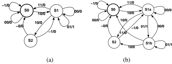
Fig. 3. FSM transformation: (a) Mealy, (b) Locally Moore.
