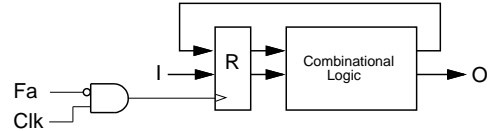
Fig. 2. Example of gated-clock FSM.
