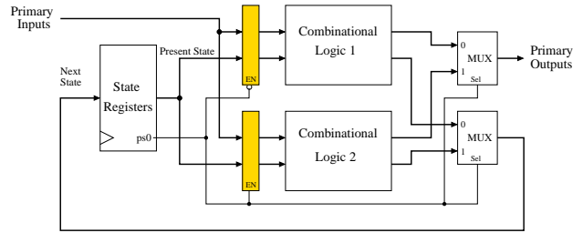
Fig. 5. Partitioning the encoding of states.
