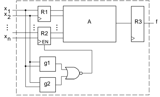
Fig. 1. Precomputation architecture.
