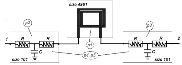
Fig. 2. Interconnection scheme for Example 1, with original sizes and parameter indication.
