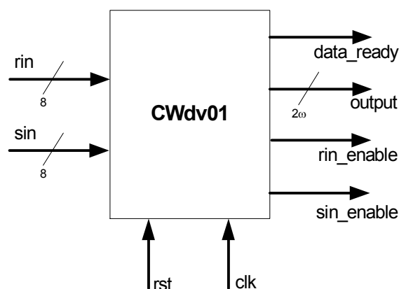
Figure 1. CWdv01 symbol and interface signals.
