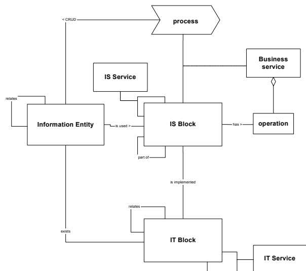
Figure 2. Proposed meta-model profile (level 0)
