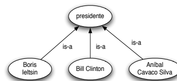
Figure 1: is-a relations
